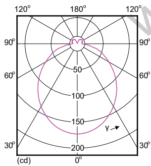
CLA LEDspotMV ND 5W PAR16 GU10 865 520lm
