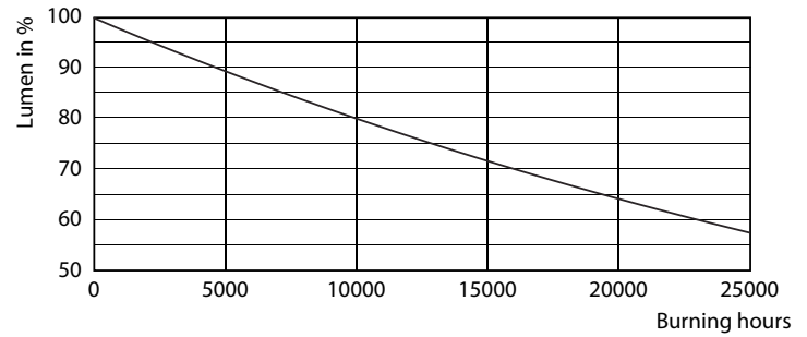
CLA LEDspotMV 50W GU10 827 36D ND
